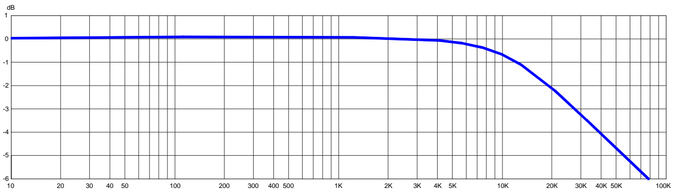
AT-100L FREQUENCY RESPONSE AT 8 OHM RESISTOR LOAD
