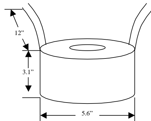
Weight = 12 LB
