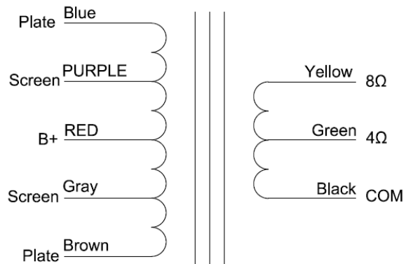
Antek MP-15W75: 12AX7 Driving 2x EL84 into 8 Ohms
