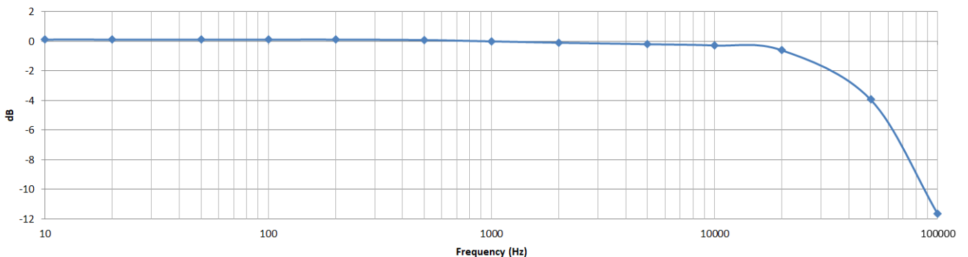
Antek MP-15W75: 12AX7 Driving 2x EL84 into 8 Ohms
