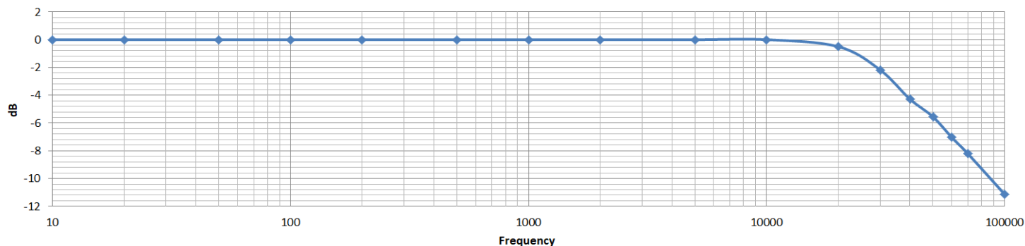
Frequency Response with 8 ohm Load
