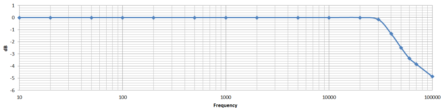
Frequency Response with 8 ohm Load
